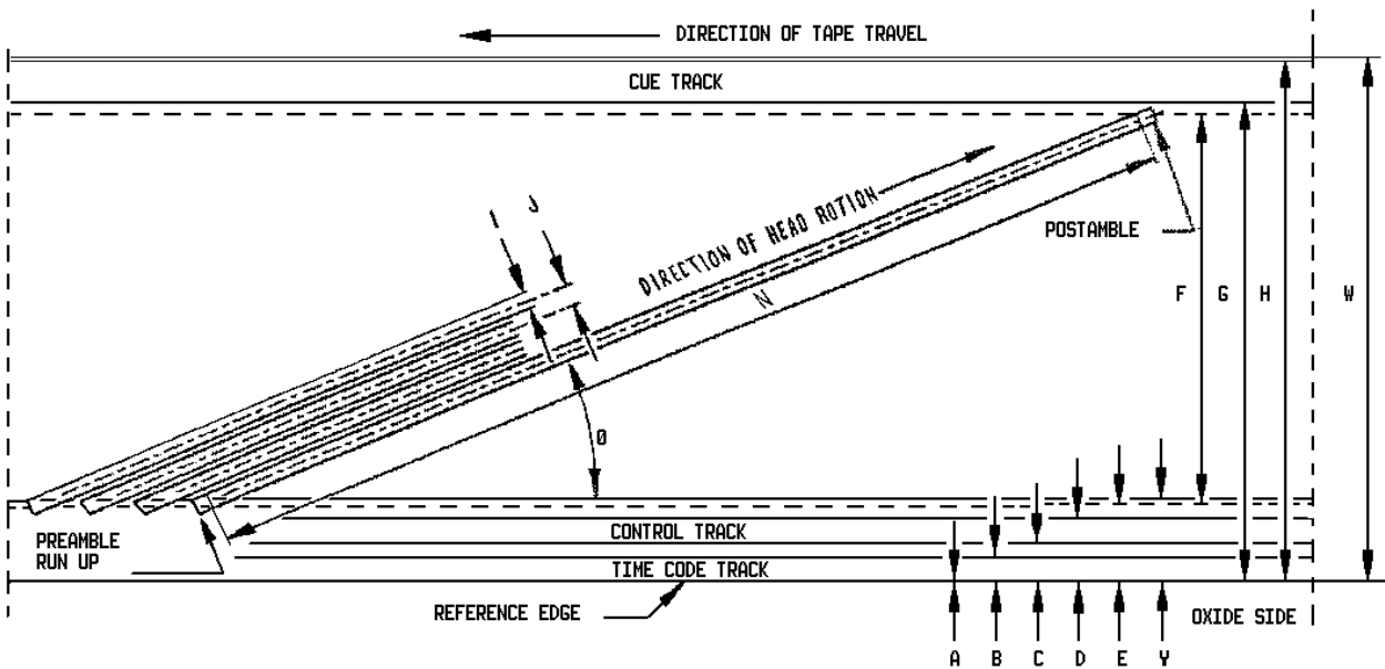
Diagram showing the track layout on the tape.
